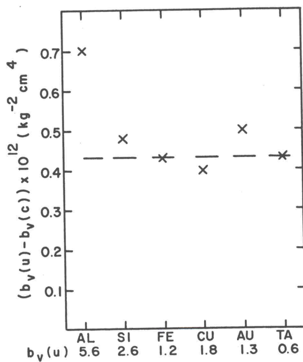
Fig. 3. Difference between ultrasonic and compression values of b_v for several incompressible elements. Dashed line represents the zero of ordinate corresponding to the correction proposed by Rotter and Smith (1) .
